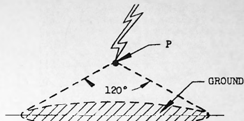
FIGURE 7-A. LIGHTNING PROTECTIVE ZONE CREATED BY A SINGLE CONDUCTIVE POINT, P, SUITABLY GROUNDING
