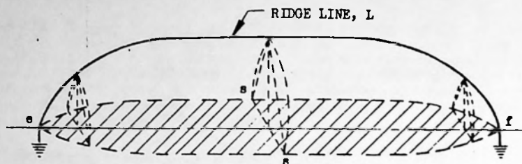
FIGURE 8-A. PROTECTIVE ZONE CREATED BY A SINGLE GROUNDED CONDUCTOR, L, LAID CENTRALLY OVER RIDGE OF TYPICAL DIELECTRIC CANOPY OR BLISTER. (THIS ZONE MAY BE CONSIDERED AS DEVELOPED BY A COMBINED RADIAL AND TRANSLATORY MOTION OF THE APEX, FROM e TO f)
