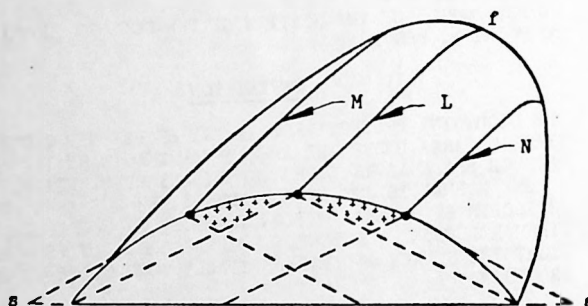
FIGURE 8-C. PERSPECTIVE OF SECTION s-f-s SHOWN IN FIGURES 8-A AND 8-B, SHOWING HOW A COMPOUND PROTECTIVE ZONE MAY BE BUILT UP BY INSTALLATION OF ADDITIONAL GROUNDED CONDUCTORS, M AND N, WHICH PRODUCE OVERLAPPING PROTECTIVE ZONES
