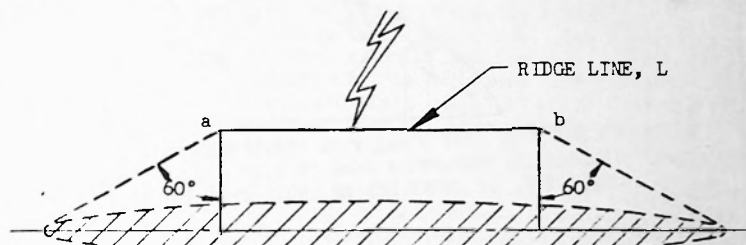
FIGURE 7-B. PROTECTIVE ZONE CREATED BY A CONDUCTIVE RIDGE LINE, L, SUITABLY GROUNDING. (THIS ZONE MAY BE CONSIDERED AS DEVELOPED BY A SIMPLE MOTION OF TRANSLATION OF THE CONE IN FIGURE 7-A FROM POINT a, TO POINT b, ABOVE)
