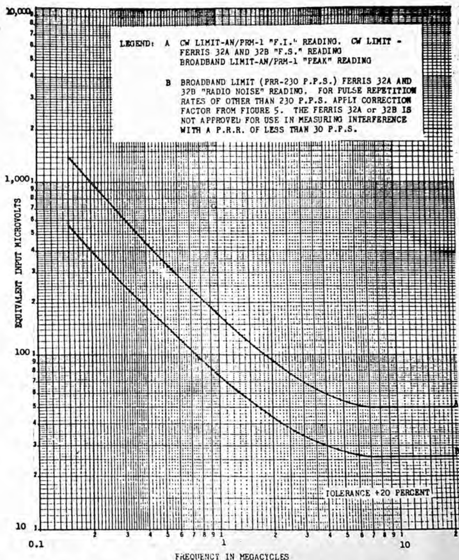
FIGURE 1. Conducted interference limits - broadband and cw
