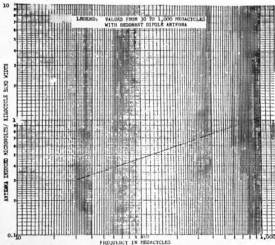
FIGURE 17. Standard limits broadband radiated interference
