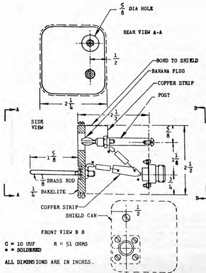
FIGURE 15. Drawing of a matching connector for use with the Ferris meter
