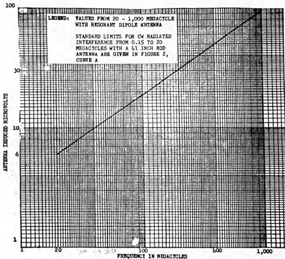
FIGURE 18. Standard limits cw radiated interference
