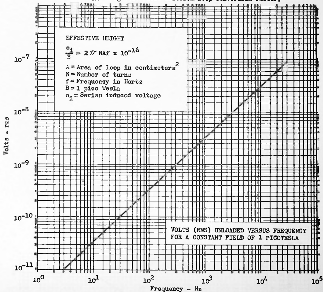
FIGURE 10- Magnetic field emission loop conversion factor.
