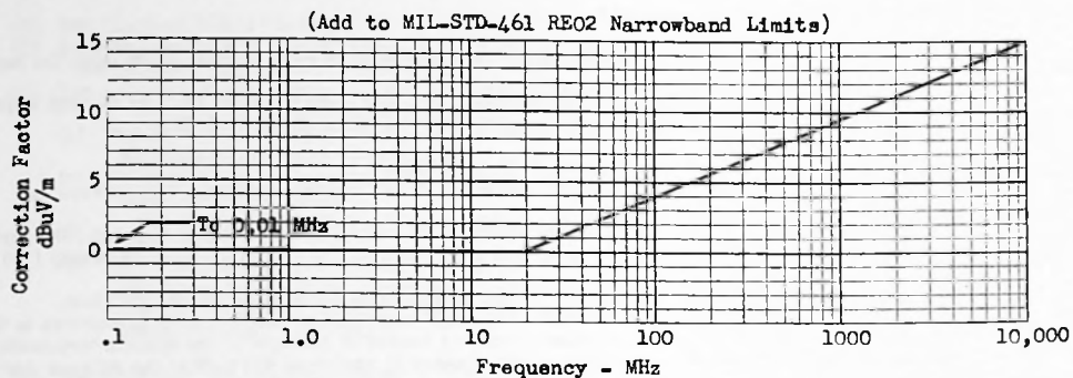
FIGURE A-1b: MIL-E-55301 and MIL-I-11748
