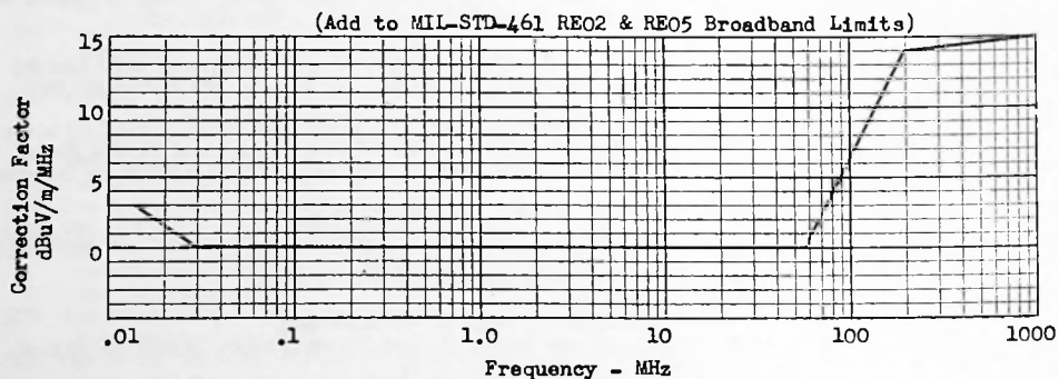
FIGURE A-1c: MIL-I-16910C and MIL-I-17623A
