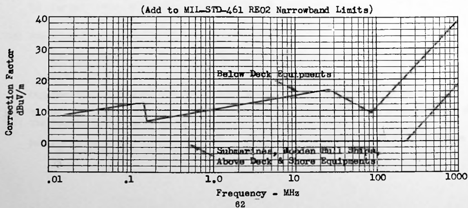
FIGURE A-1c: MIL-I-16910C and MIL-I-17623A
